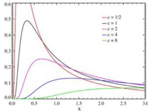
Figure 1: Levy distributions for different values of the scale parameter c
